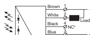
*Do not connect black wire SMP / SMPF / SMRR 7600 (load as NPN)
