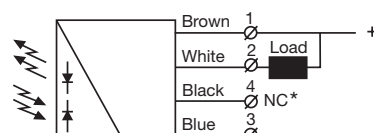
SPRR / SPPR / SPP / SPBS 26xx (load as NPN)
