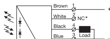
SPRR / SPPR / SPP / SPBS 26xx (load as PNP)
