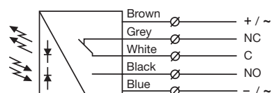
SPRR / SPPR / SPP / SPBS 29xx
