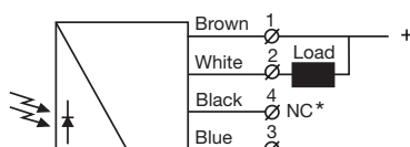
SPR 2645 (load as NPN)
