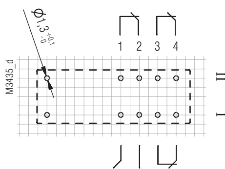
Pin arrangements OA 5611.28 1NO / 3NC
