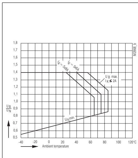
Operating voltage limit curve OA 5612
