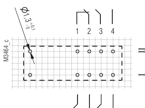
Pin arrangements OA 5611.48/...L4 3NO / 1NC
