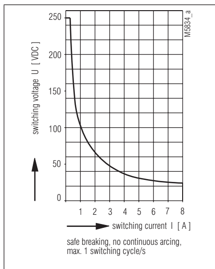
Limit curve for arc-free operat. (load limit curve)
