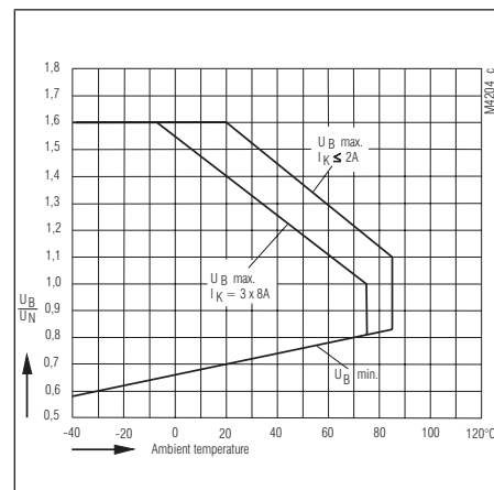
Operating voltage limit curve OA 5644.48
