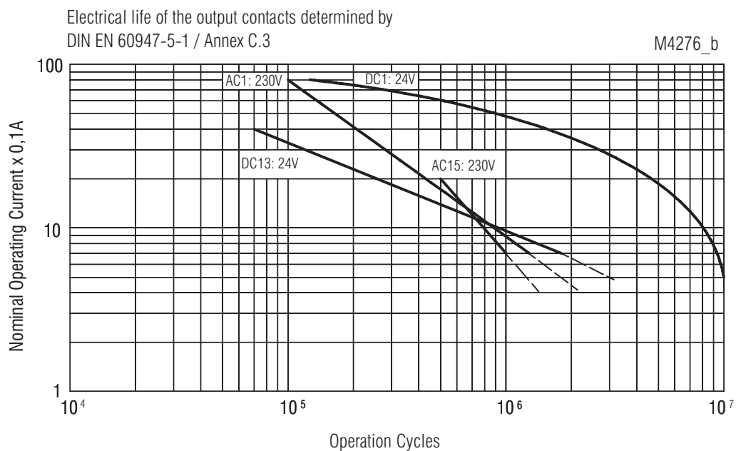
Electrical life
