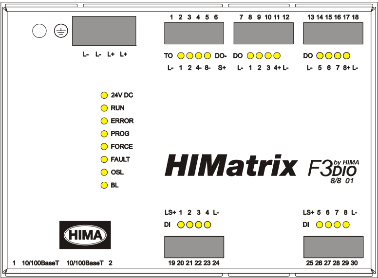
Figure 6: Front View
