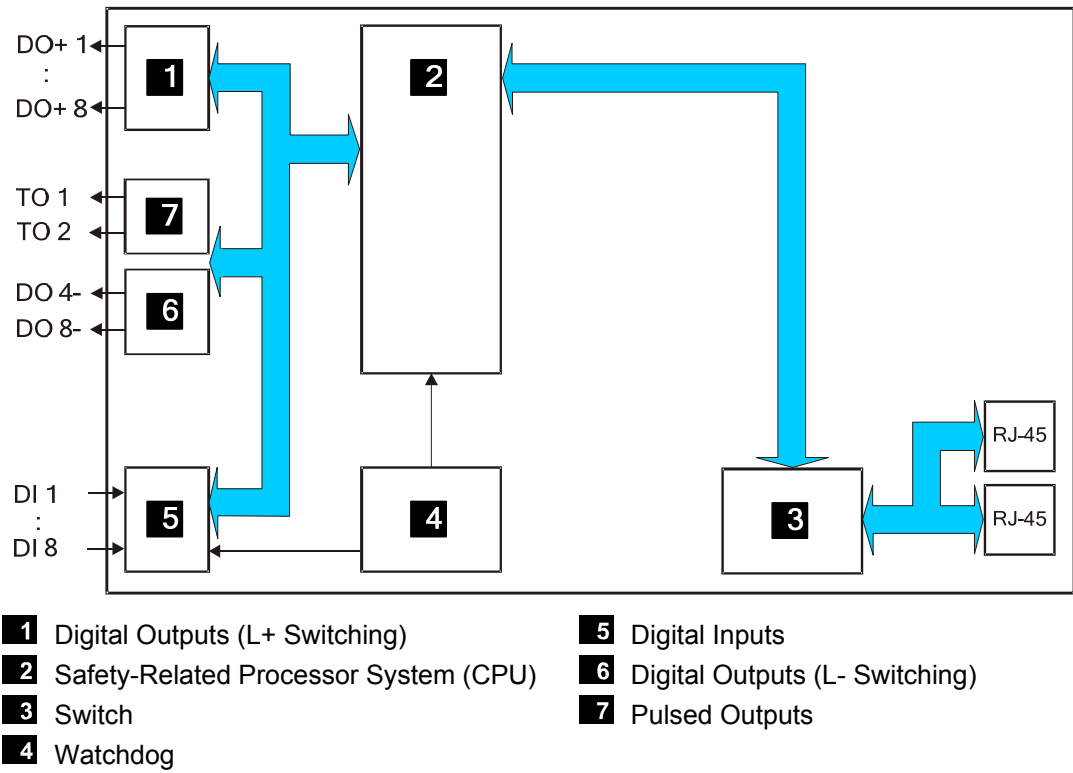
Figure 7: Block Diagram
