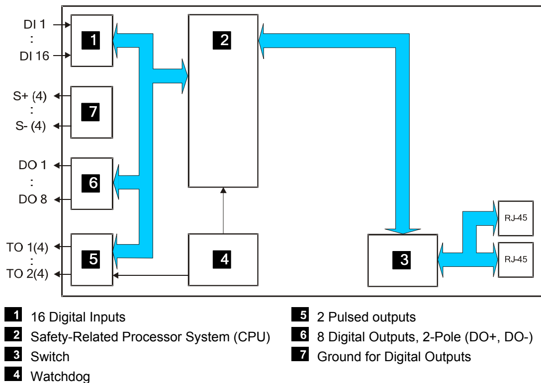
Figure 8: Block Diagram
