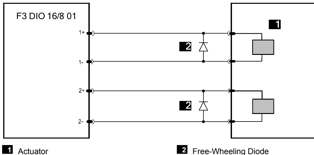
Figure 12: 2-Pole Connection of an Actuator
