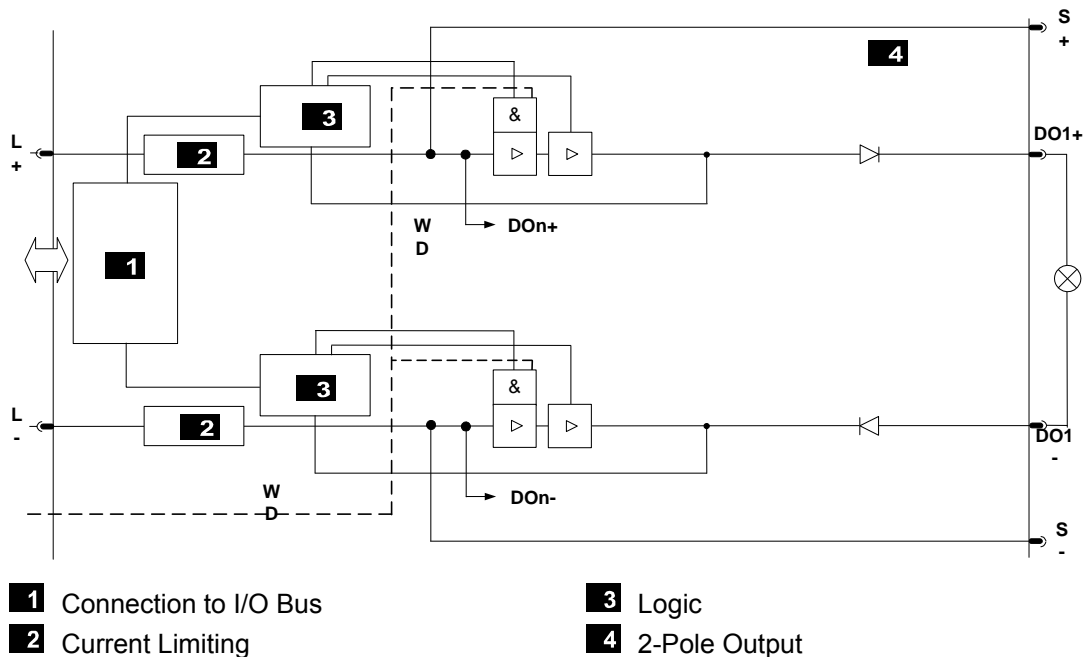
Figure 5: Block Diagram for 2-pole Digital Outputs
