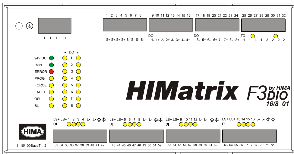
Figure 7: Front View
