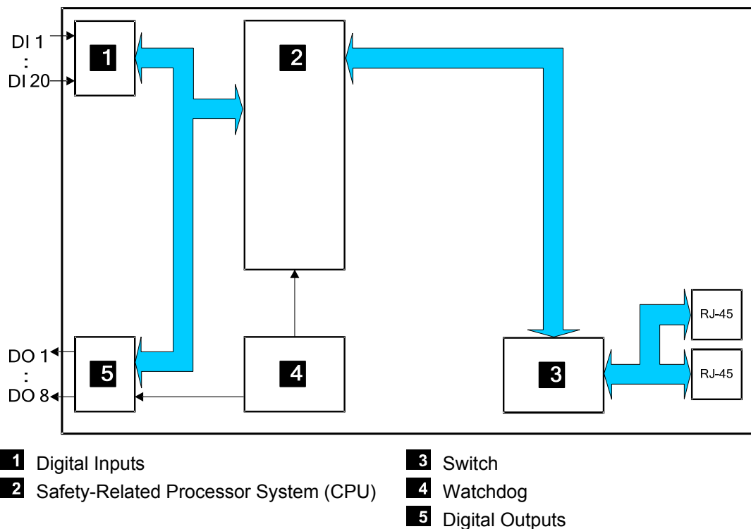
Figure 6: Block Diagram
